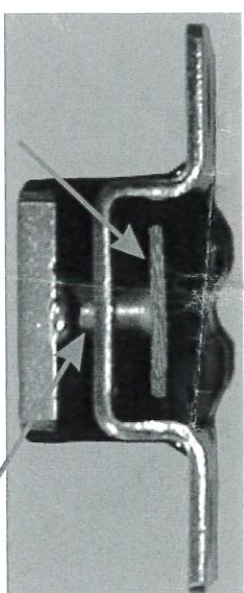
Side view (cutaway) showing safety interlock
