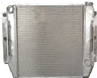
This cross-flow aluminum radiator was configured for the Novak LS1 TJ project, and is an example of an excellent cooling solution, critical with such a fine and expensive motor in the bay.
